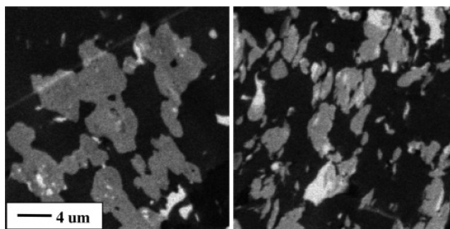
Figure 11. Scanning transmission X-ray microscopy (STXM) images (20 \mu\text{m} \times 20 \mu\text{m} ) of PS/PVC blends (taken at 285.2 eV, the absorption energy of PS, PS is dark): (a) PS/PVC (50/50), (b) PS/PVC/Cloisite 6A (45/45/10).
